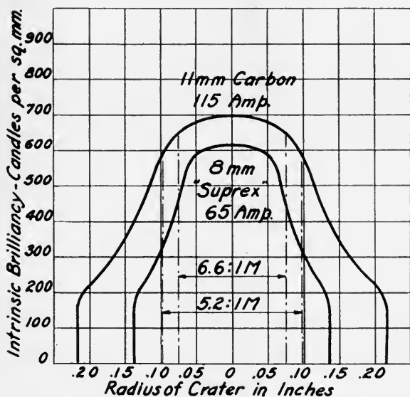
FIG. 2. Comparison of the intrinsic brilliancy and size of the crater of the 8-mm "Suprex" positive at 65 amperes in a horizontal trim, and the 11-mm carbon at 115 amperes in an angular trim.
